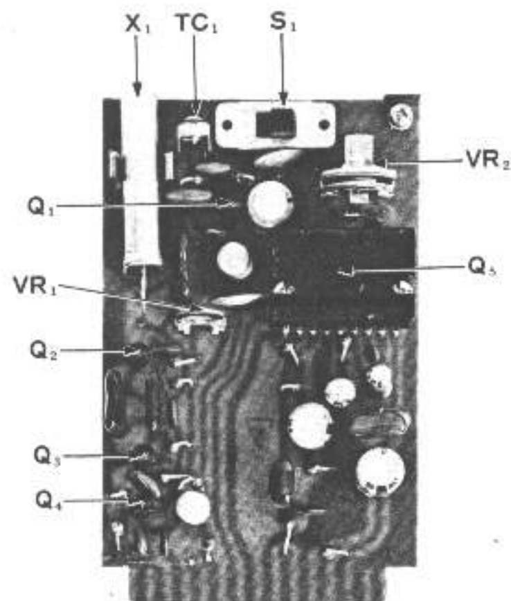
Fig. 16 AF-CALIB UNIT
