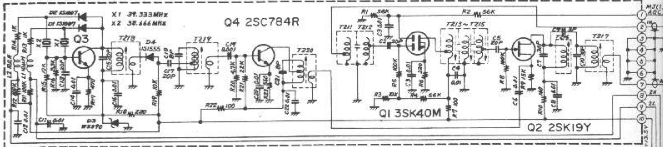
PB-1305A(6m CONVERTER)
