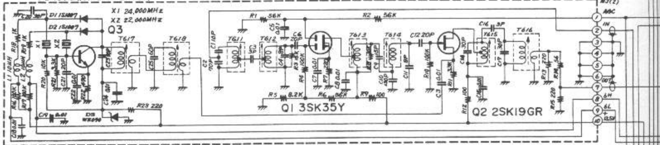
PB-1305A(6m CONVERTER)
